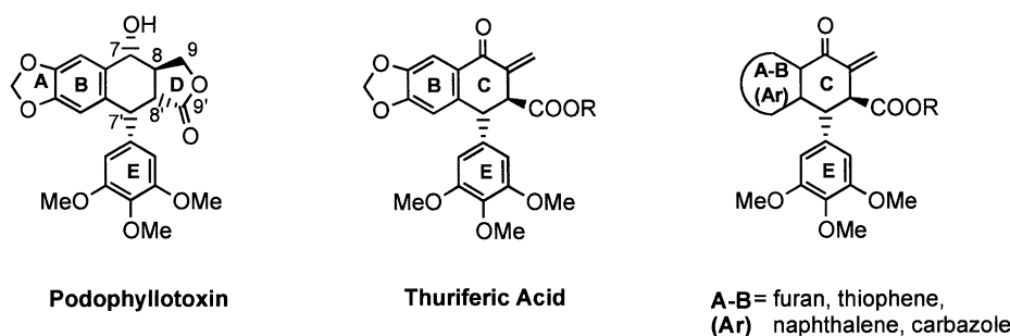
Figure 1. Structure of model lignans and synthesised compounds.
