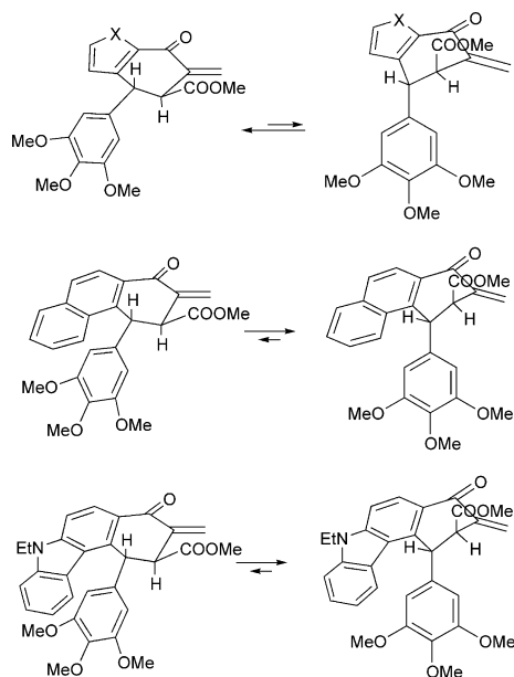
Figure 4. Conformational equilibrium of thiophene and furan, naphthalene and carbazole analogues of thuriferic acid.
