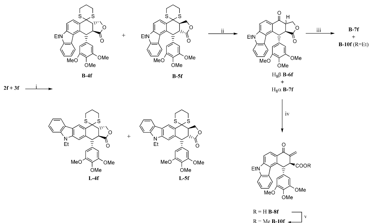
Figure 3. Synthesis of carbazole analogues. Key: (i) TFA, CH 2 Cl 2 , 24 h. (ii) HgO, BF 3 ·Et 2 O, THF–H 2 O (85:15), 0 °C → rt, 24 h; (iii) EtOH/HOAc, reflux, 48 h. (iv) 1% KOH/MeOH, rt, 1.5 h; then HCl 2 N. (v) ethereal CH 2 N 2 .
