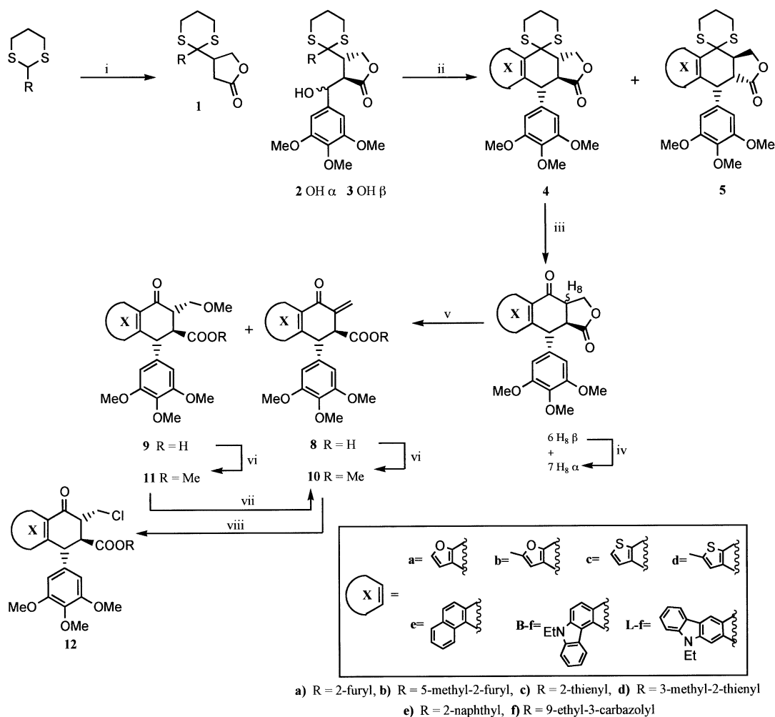
Figure 2. General synthesis of thuriferic acid analogues and their derivatives. Key: (i) (a) BuLi 1.6 M, THF, -78^{\circ}\text{C} , 45 min; (b) 5 H -furan-2-one, THF, -78^{\circ}\text{C} , 3 h; (c) Ar-CHO, THF, TMEDA, -50^{\circ}\text{C} , 12 h. (ii) TFA, \text{CH}_2\text{Cl}_2 , 24 h. (iii) \text{HgO} , \text{BF}_3 \cdot \text{Et}_2\text{O} , THF– \text{H}_2\text{O} (85:15), 0^{\circ}\text{C} \rightarrow \text{rt} , 24 h; (iv) EtOH/HOAc, reflux, 48 h. (v) 1% KOH/MeOH, rt, 1.5 h; then HCl 2 N. (vi) ethereal \text{CH}_2\text{N}_2 . (vii) p -TsOH, \text{C}_6\text{H}_6 , reflux, 7 h. (viii) HCl dry stream, \text{CH}_2\text{Cl}_2 , 2 h.
